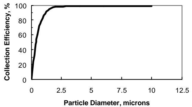
Fig.3. ESP Collection Efficiency
