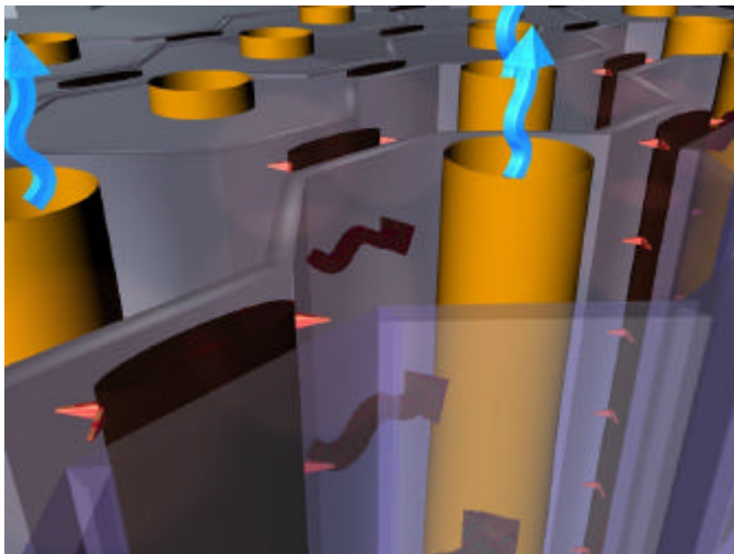
Fig. 4. MSC Arrangement (Artist's Rendition)
