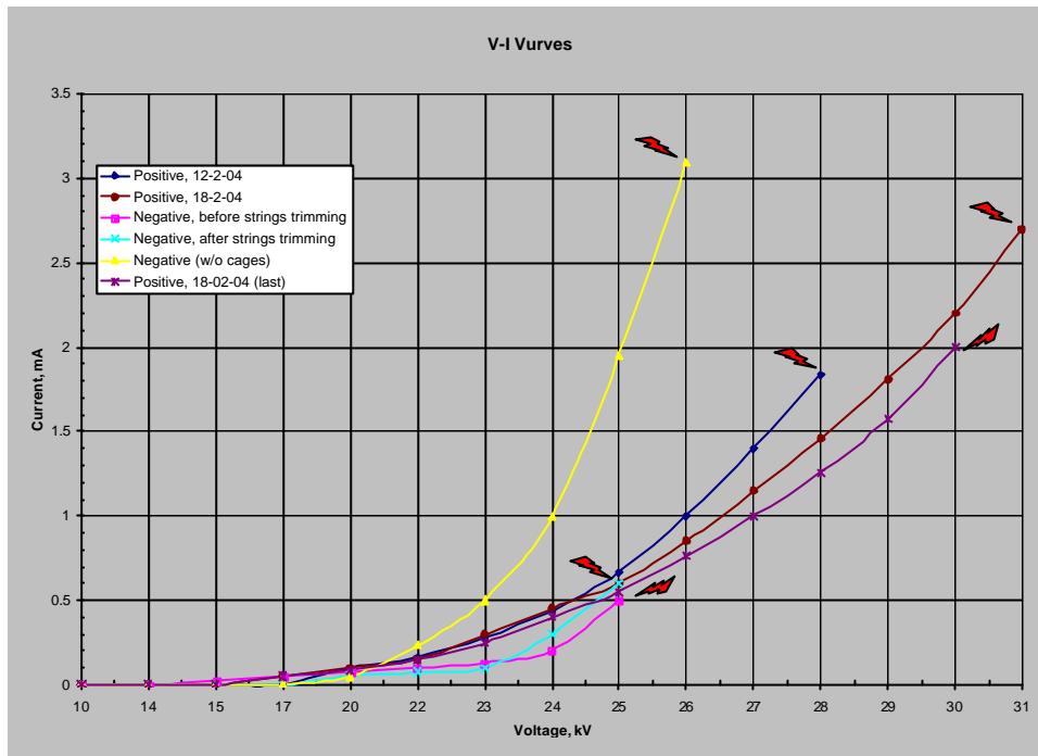
Fig. 12. Demonstration MSC™ Electrical Clearances Evaluation
