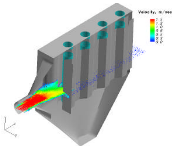
Fig. 10. CFD Simulation
