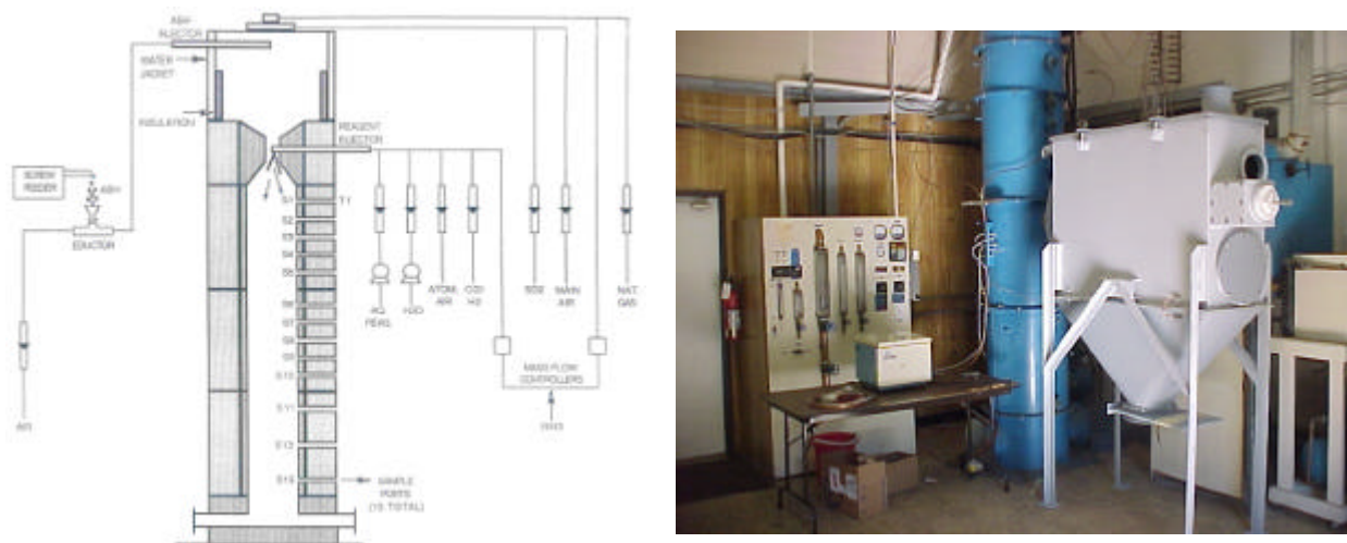
Fig. 7. Pilot-Scale Apparatus: Combustor, MSC TM and Ancillary Equipment
