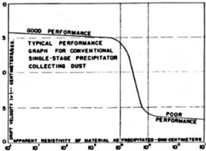
Fig. 2. "Conventional" Precipitator Migration Velocity Relationship
