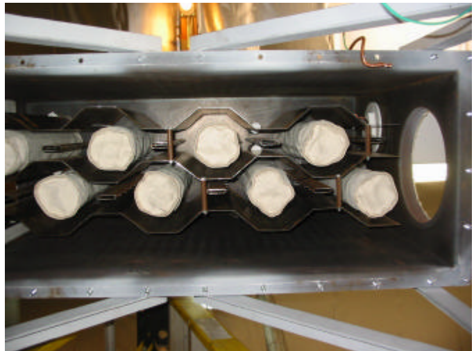
Fig. 6. View into Bottom of the Pilot MSC Unit
