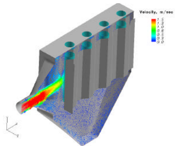
Fig. 11. Gas Recirculation in the Hopper
