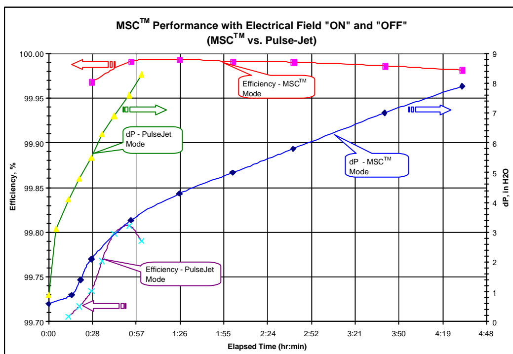
Fig. 14. MSC™ POC Pilot Performance
