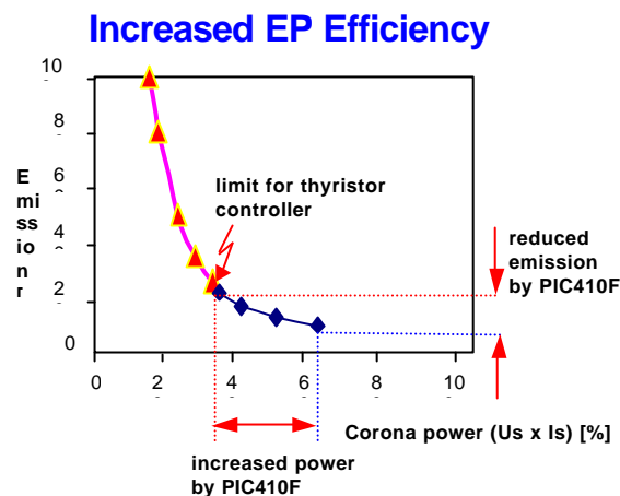
Figure 5: Emission over power
