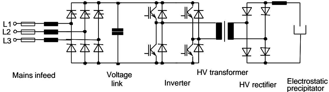
Figure 1: Basic IGBT inverter circuit
