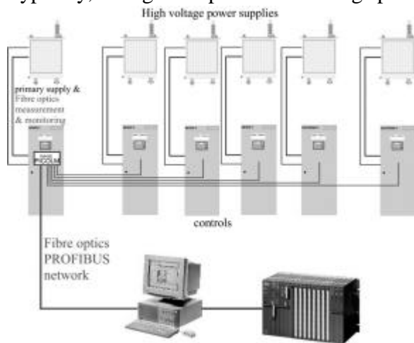
Fig. 8: Power control system "WINPIC"
