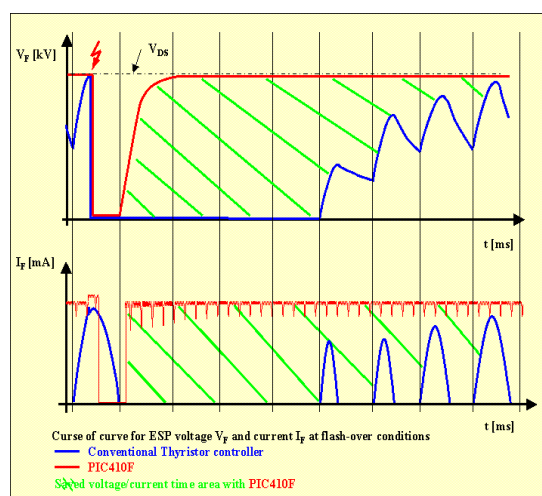
Figure 2: precipitator voltage and current
