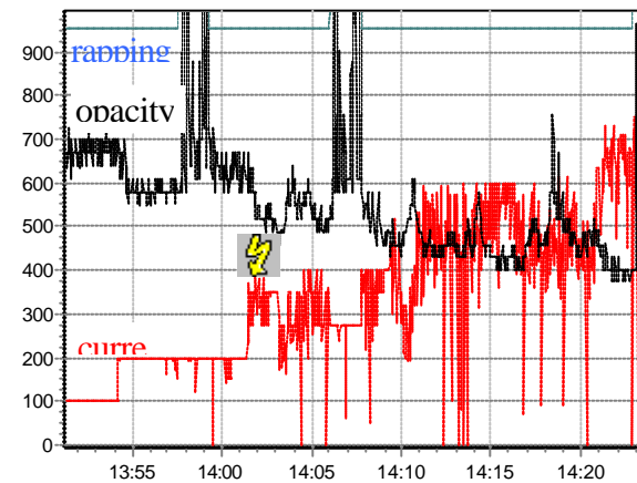
Figure 6. opacity and current – inlet field
